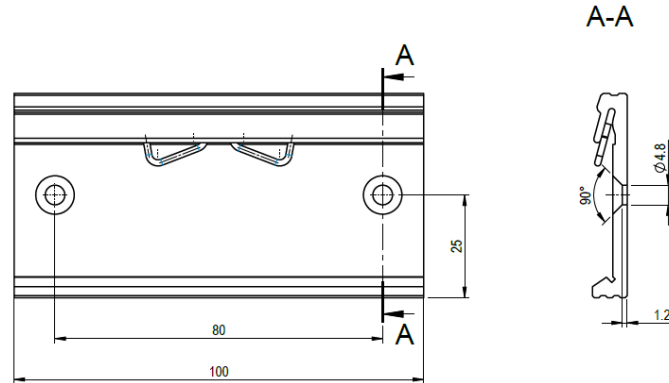
Figure 2: Mechanical dimension of adapter board (optional accessory).
